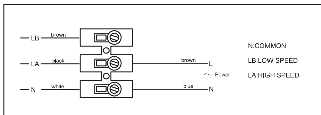
Wiring with speed control
