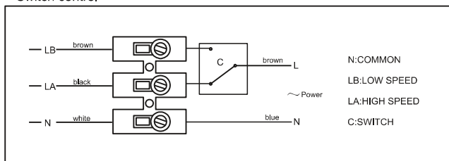
Switch control
